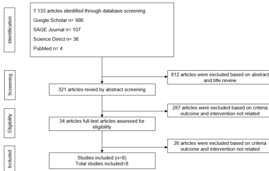
Figure 1: PRISMA Diagram
